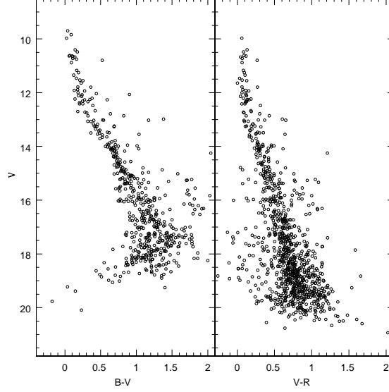
Figure 3. The color-magnitude diagram of the star cluster M 36 observed in BVR on 30th November 2010 from 1.3m DFOT at Devasthal, Nainital.
