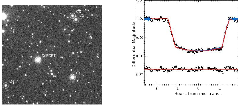
Figure 4. The R-band image (left) and differential light curve (right) of the transiting extrasolar planet WASP12 ( V \sim 11.7 mag star) observed on 5 th February 2011 with the 1.3-m DFOT at Devasthal, Nainital. The image is exposed for 5s and it covers about 6' on a side. The target and the four comparison stars are encircled. Each single data point in the light curve represents flux from twenty coadded frames. The model is overplotted and a typical error in each data point is of the order of 1 mmag.
