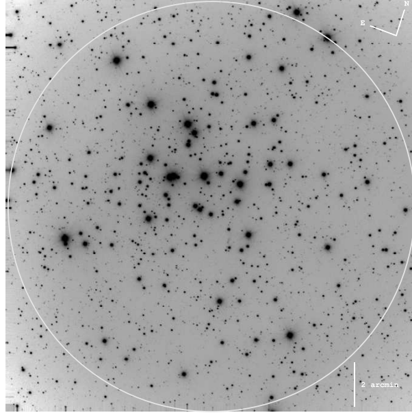
Figure 2. The R-band image of the star cluster M 36 taken on 30th November 2010 from 1.3m DFOT at Devasthal-Nainital. The image is a 45 co-added frames of 10s each, covers about 18' on a side and the FWHM seeing is about 2". The unvignetted field of view is shown in circle.
